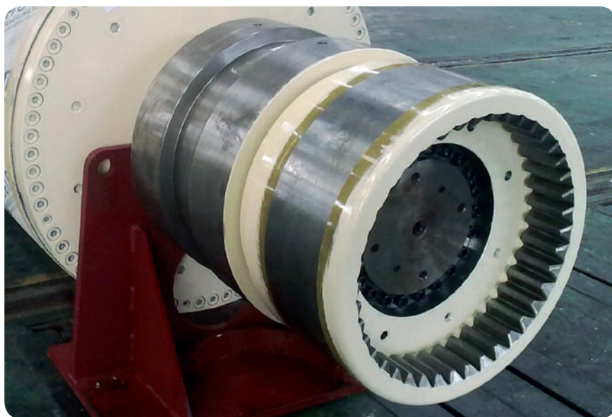
SKF FX Keyless Bushing PHF FX60-320X405 was installed on heavy duty paper roll application.
